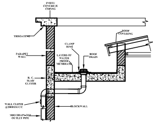
TYPICAL DRAIN-OFF DETAIL A @ EAVES
