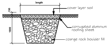
SECTION D - D
