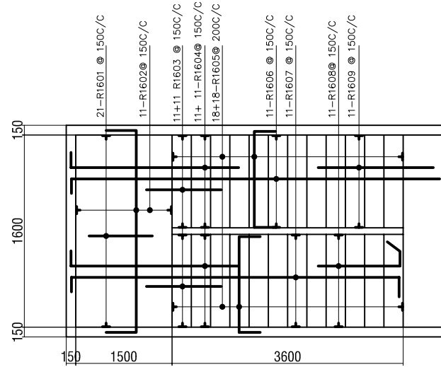
R.C STAIR CASE FROM SECOND FL. TO THIRD FLOOR
