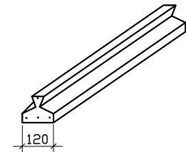
T4 PRESTRESSED CONCRETE JOIST [ scale = 1:50mm ]
