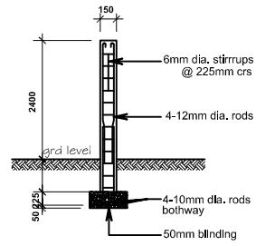
COLUMN SECTION
