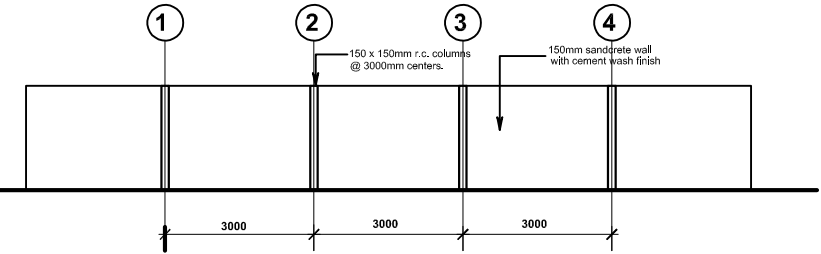
ELEVATION (side wall)
