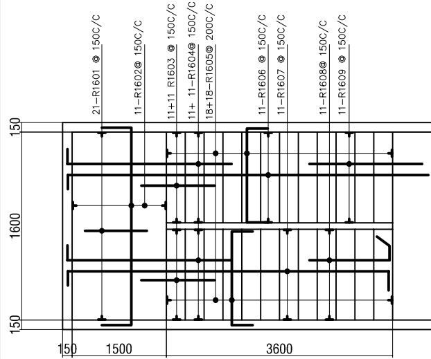
R.C STAIR CASE FROM GROUND FL. TO FIRST FLOOR
