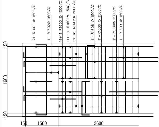
R.C STAIR CASE FROM FIRST FL. TO SECOND FLOOR
