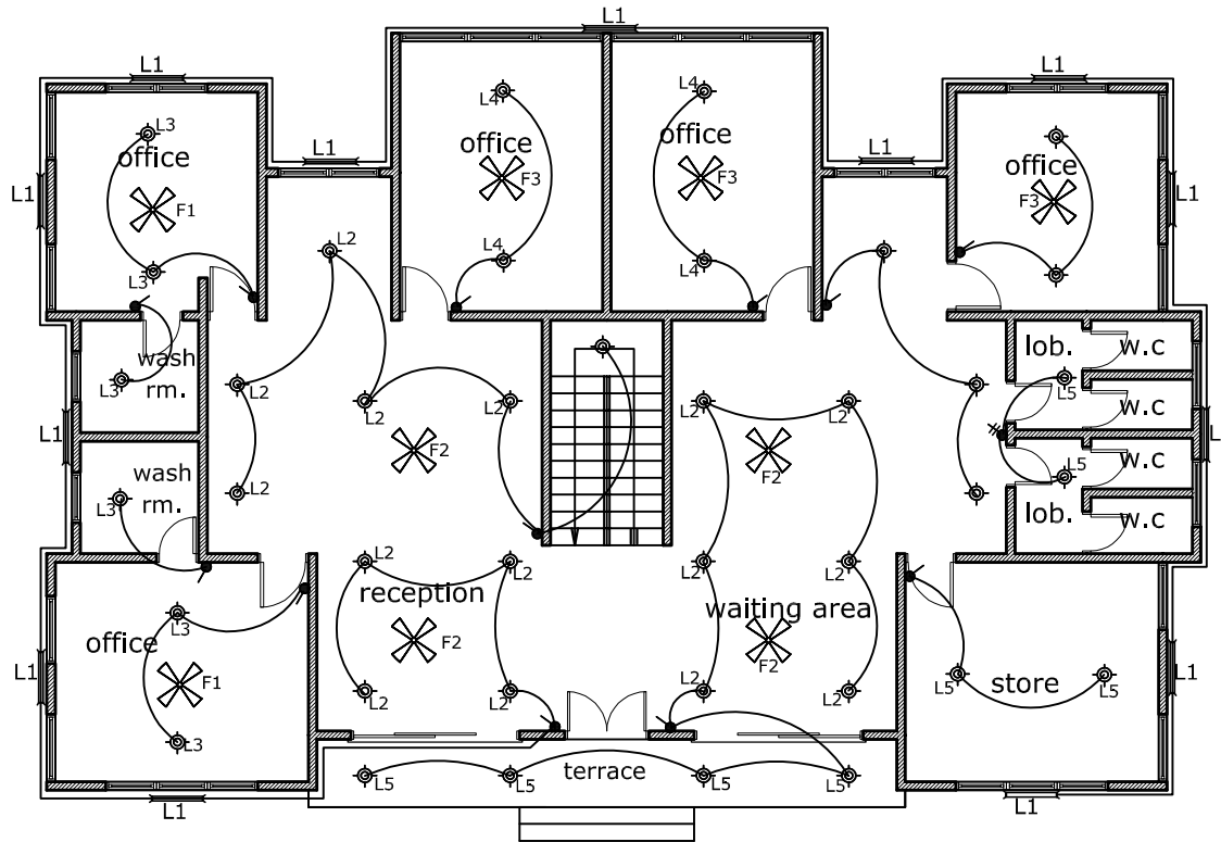
GROUND FLOOR ELECTRICAL LAYOUT SCALE 1:100
