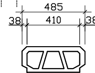
FRONT VIEW OF H16-HOLLOW BLOCK [ scale = 1:50mm ]
