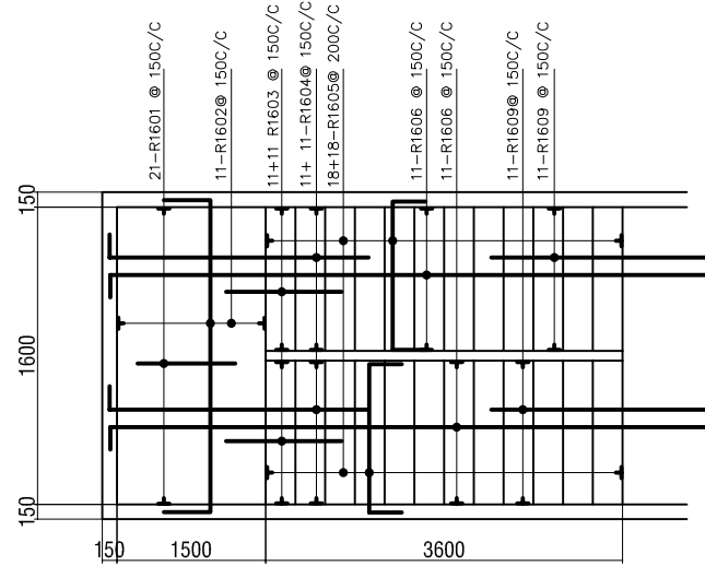
R.C STAIR CASE FROM THIRD FL. TO FOURTH FLOOR
