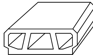
H16- HOLLOW-POT BLOCK [ scale = 1:50mm ]
