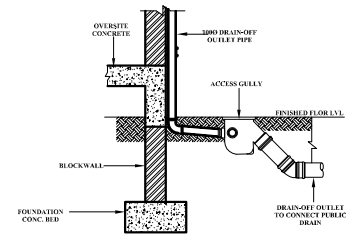
TYPICAL DRAIN-OFF DETAIL B @ FLINTH BASE
